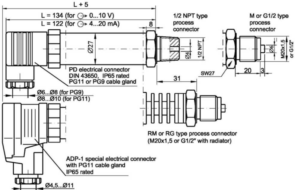
Fig.1. AS series pressure transmitter.
